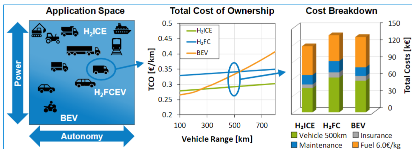
FIGURE 17: RANGE AND TCO COMPARISON FOR ZERO-CARBON POWERTRAINS 9
